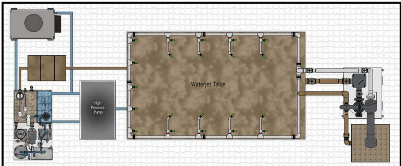
Abrasive Removal Typical Installation Shown with Closed Loop Filtration
